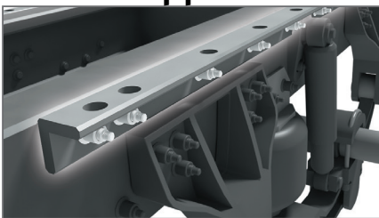
Fifth Wheel Assembly
