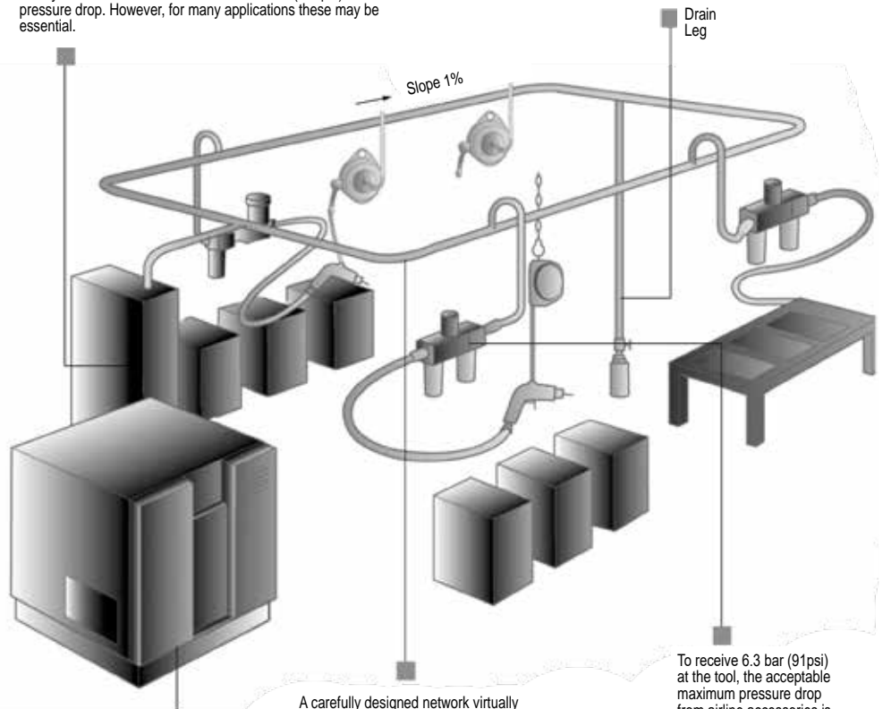
A carefully designed network virtually eliminates pressure drop. We recommend a Ring Main layout which has a slope away from the input of 1%.
