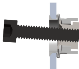
CROSS SECTION OF RIV-FLOAT®-SHORT Installed
