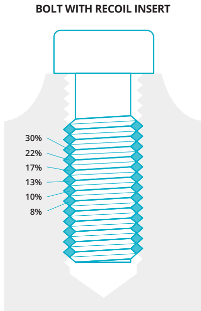
High strength: Stress spread more evenly
