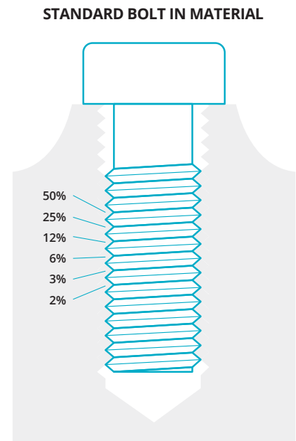
Lower strength: Stress concentrated on first threads
