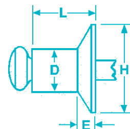
Countersunk
