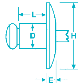
Large Flange
