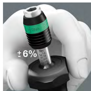
Measurement accuracy is \pm 6\% in accordance with the standard DIN EN ISO 6789. Distinctly audible and noticeable excess-load signal when the pre-set torque is reached.
