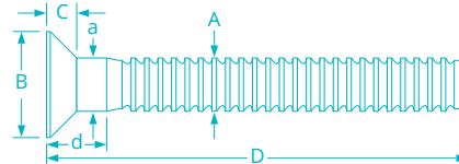
90° Flush Head MGP90
