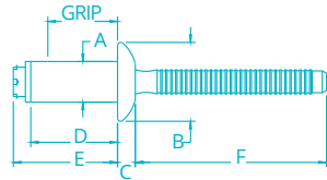
Clearance Protruding Head
