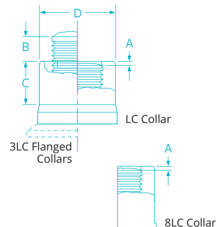
3LC Flanged Collars
