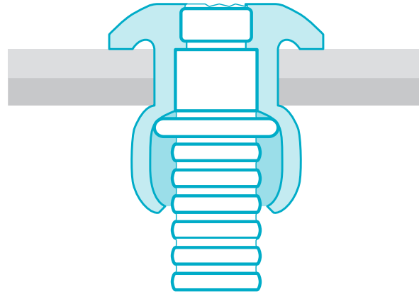
Huck Structural Blind Rivets expand or bulb on the blind side of the hole pulling the materials together and breaking the pintail flush with rivet head
