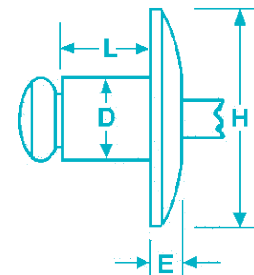
Large Flange
