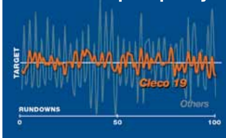
19 Series Torque Capability
