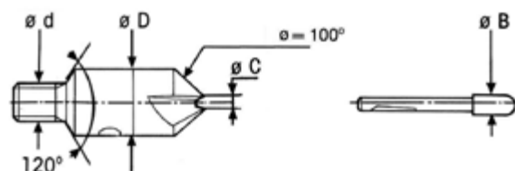
Centering cone
