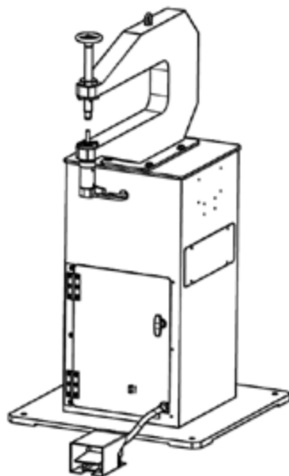
Assembly for riveting fastened to fixed frames examples
