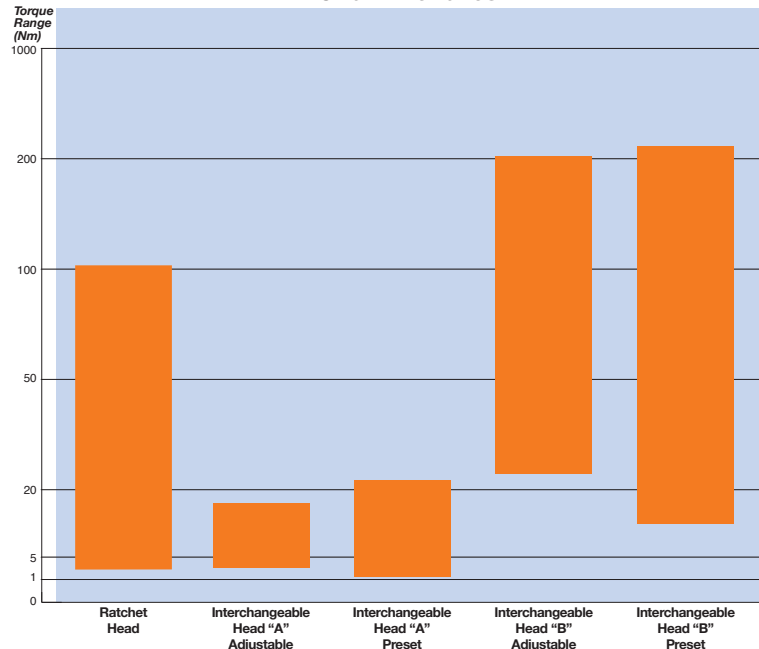
Click Wrenches
