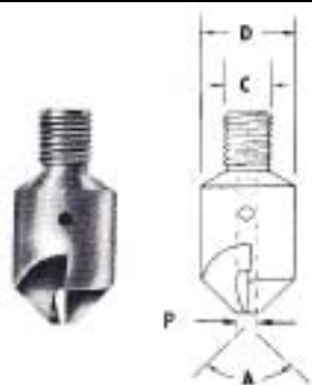
Pilot Drill Countersink Cutters
