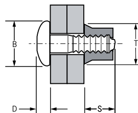
Full Collar
