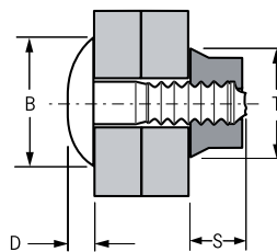
Half Collar
