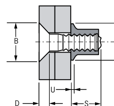
Flanged Collar
