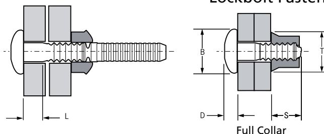
Full Collar
