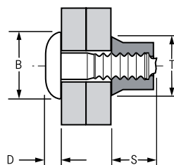
Full Collar Schließring Standard Bague Standard Collare Standard Collar Estándar
