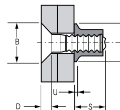
Flanged Collar
