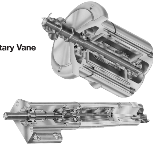
Rotary Vane
