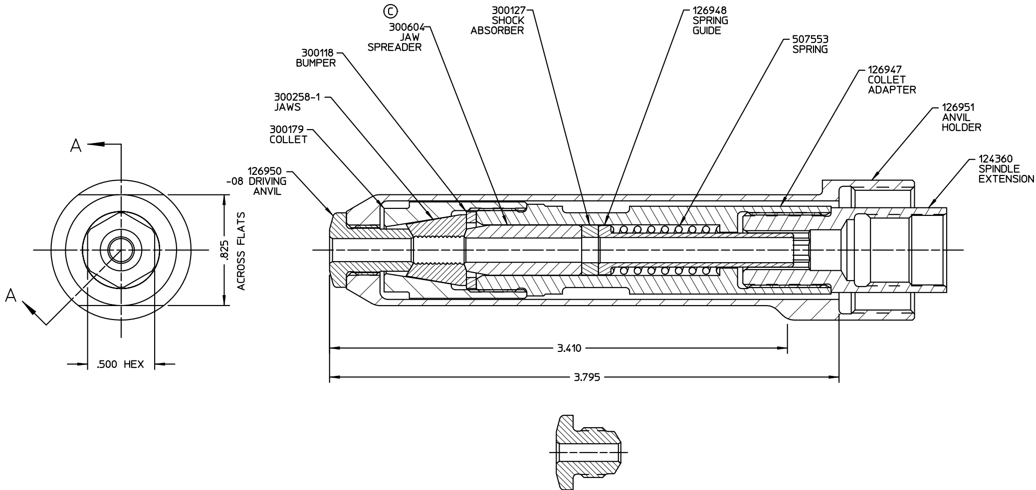
126949 -06 DRIVING ANVIL
